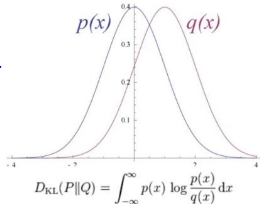
K-L Divergence
